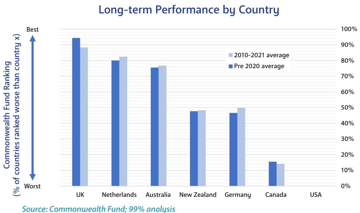
Figure 3: Rankings since 2010
